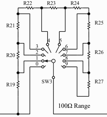
R19-R27 100R
