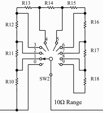
R10-R18 10R
