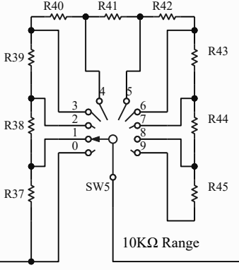
R37-R45 10K
