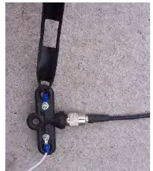
A Typical G7FEK antenna feed point before weatherproofing with self amalgamating tape
