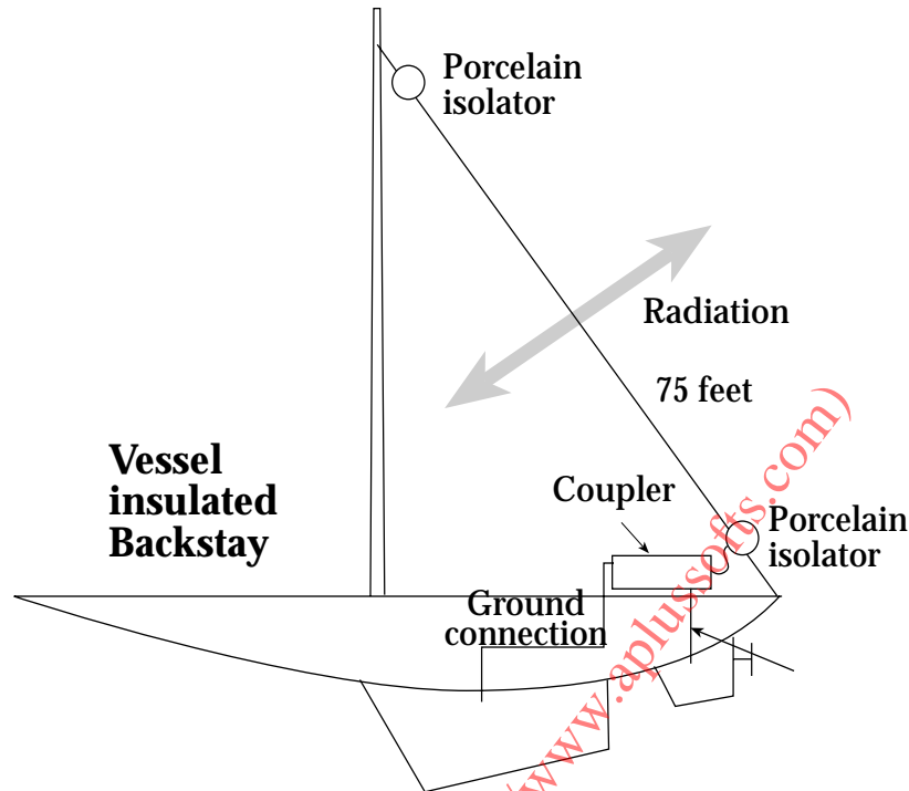
Figure 4.5.11 Vessel insulated back stay
